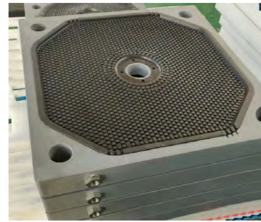
630 Diaphragm Plate
