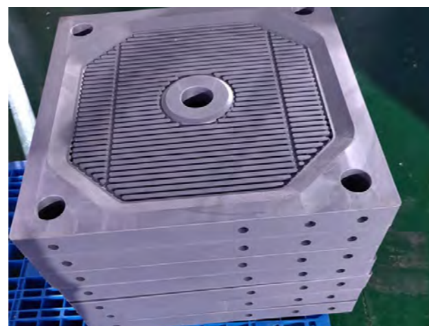
630 Filter Plate
