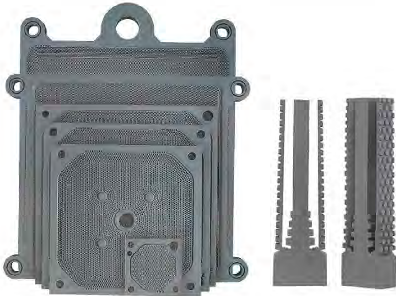
滤板系列包括250mm至2000mm不等 (该册展示不代表所有规格) Filter plate, series between 250mm-2000mm
