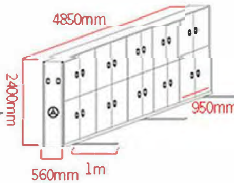
With Five bay
