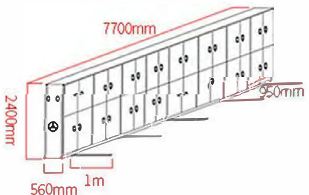
With eight bay
