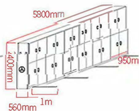
With six bay
