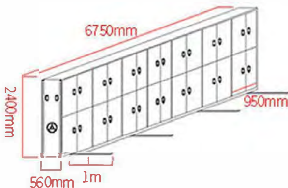
With seven bay
