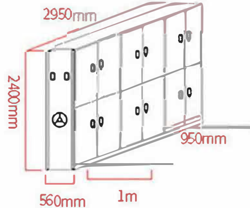
With three bay
