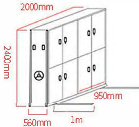
With two bay
